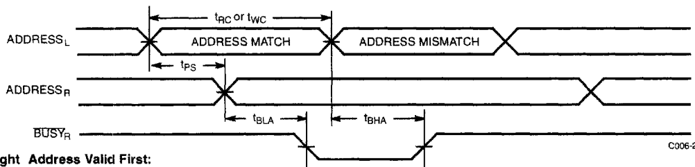
Busy Timing Diagram No.2 (Address Arbitration) [28]
